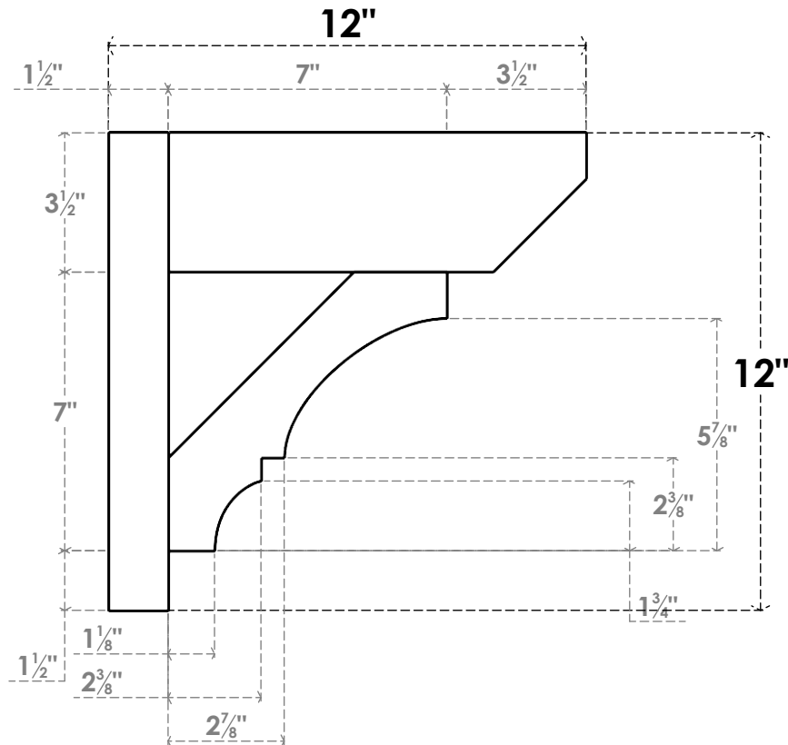
SIDE PROFILE
